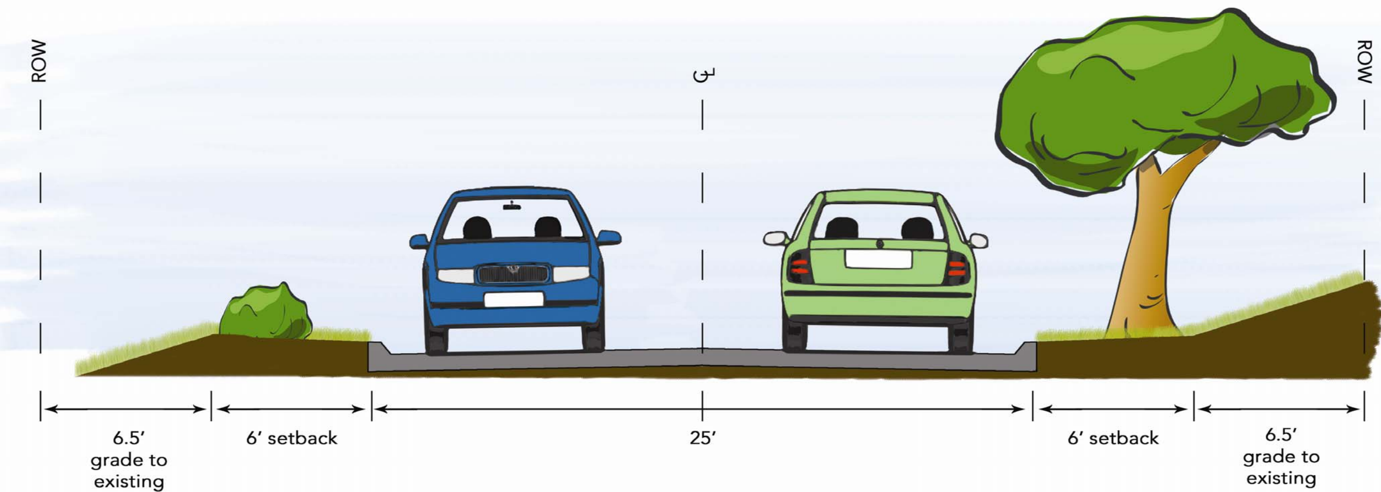
TYPICAL 2 LANE SECTION MEADOW ROAD
