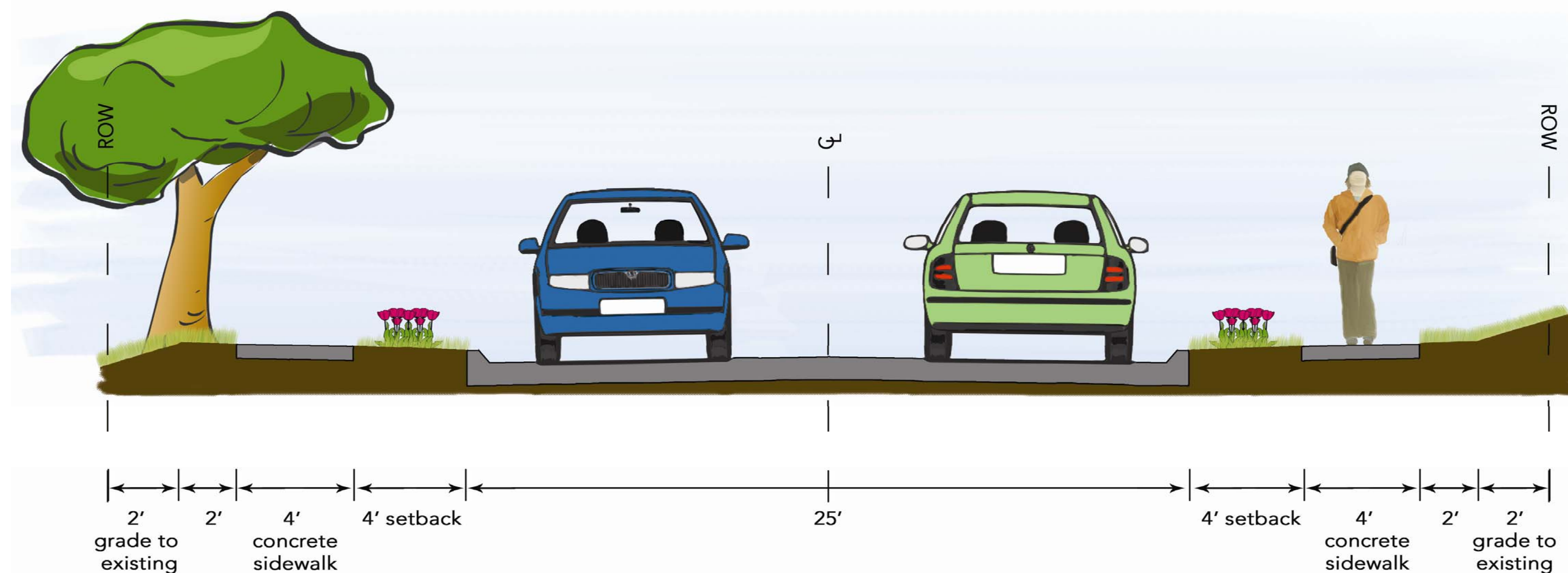
TYPICAL 2 LANE SECTION MEADOW ROAD
