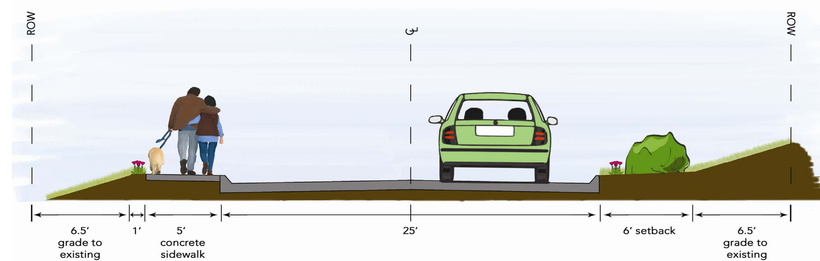
TYPICAL 2 LANE SECTION PALAMINO STREET
