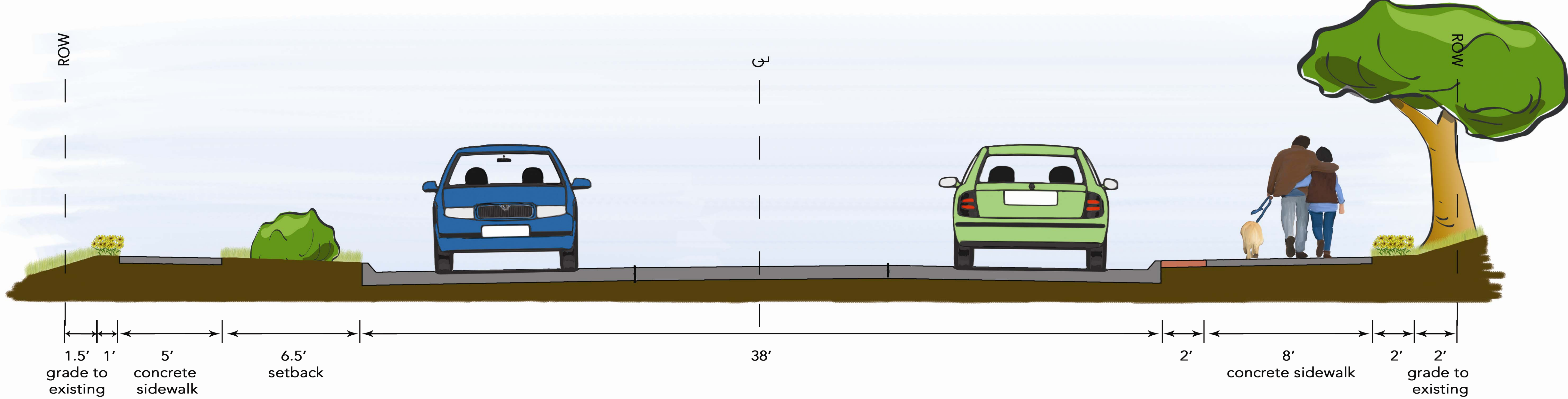
TYPICAL 3 LANE SECTION w/CENTER TURN LANE 114th STREET
