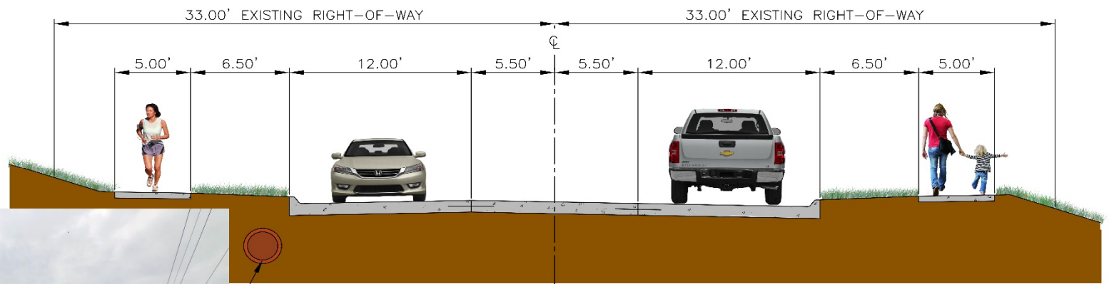
CITY OF OMAHA TYPICAL 3 LANE SECTION NO SCALE
