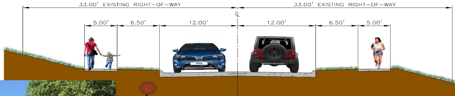
CITY OF OMAHA TYPICAL 2 LANE SECTION NO SCALE
